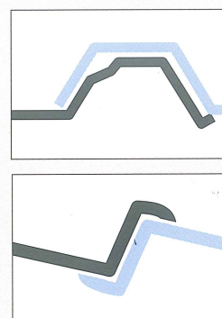
CORRECT LAP DETAIL FOR VARIOUS INFILL SHEET PROFILES
